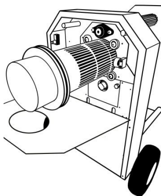
3.Once the drive belt is out, we can remove the drum by pulling it out.
