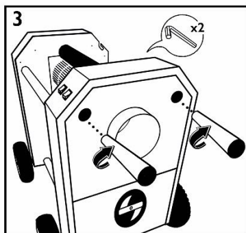
3. Place the long handles in the upper holes and collar the Allen screws
