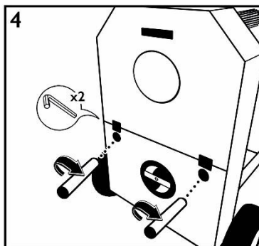
4. Place the short handles on the lower part and collar the Allen screws.
